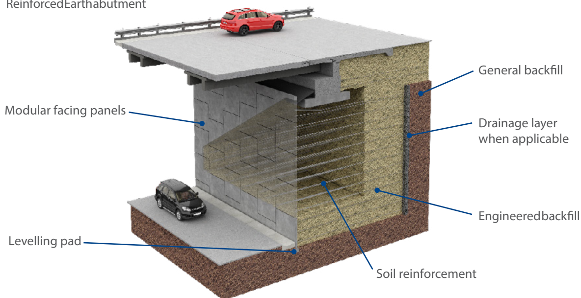
ReinforcedEarthabutment
